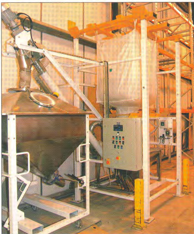
The transfer bin is mounted on a platform scale, which transmits gain-in-weight signals to a controller that runs, slows, and stops the conveyor, achieving rapid batching cycles and ±0.04 percent batch weight accuracy.
